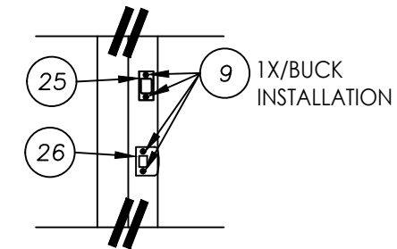
STRIKE DETAIL W/1X BUCK
