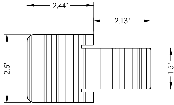
50 MULLION
