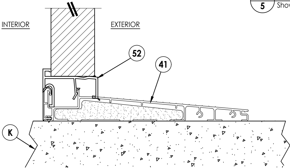
3 5 VERTICAL CROSS SECTION
