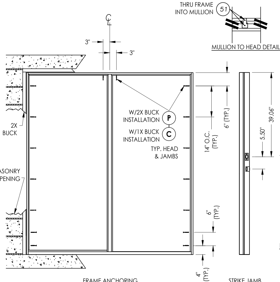
FRAME ANCHORING
