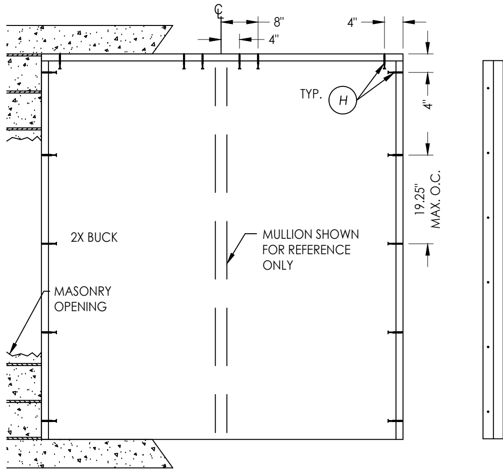
BUCK ANCHORING
