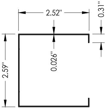
50 MULLION
